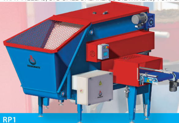
RP1 TEMPLATE FILLER UP TO 600 CONTAINERS/HOUR
