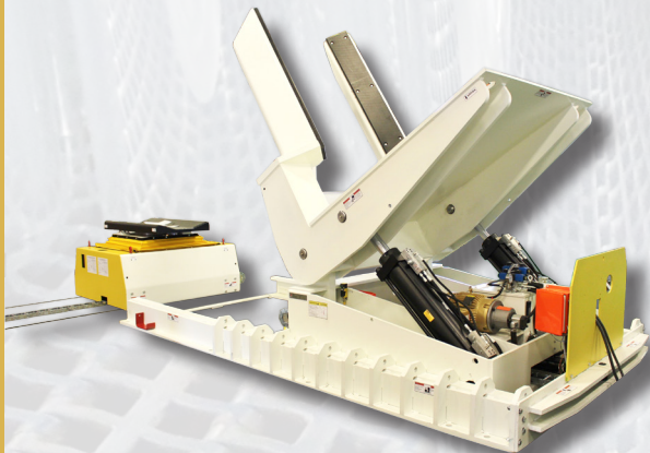
VERTICAL TAB UNCOILER
