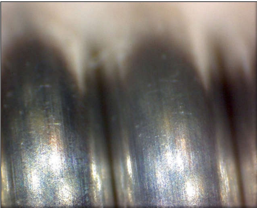
Safra ER5356 1.2 mm, mandrel test.
