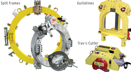
E.H. WACHS portable cutting & beveling machines
